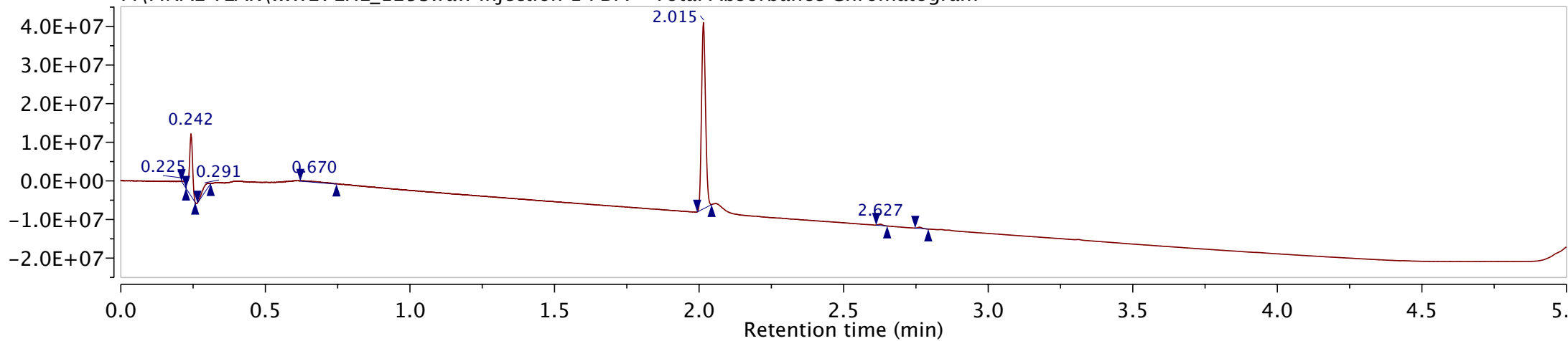
F:\FINAL YEAR\...W27LHE_1253.raw Injection 1 PDA - Total Absorbance Chromatogram
