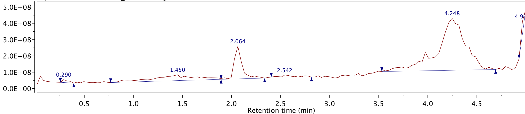
F:\FINAL YEAR\...W27LHE_1253.raw Injection 1 MS ES+ MS + spectrum 2.03
