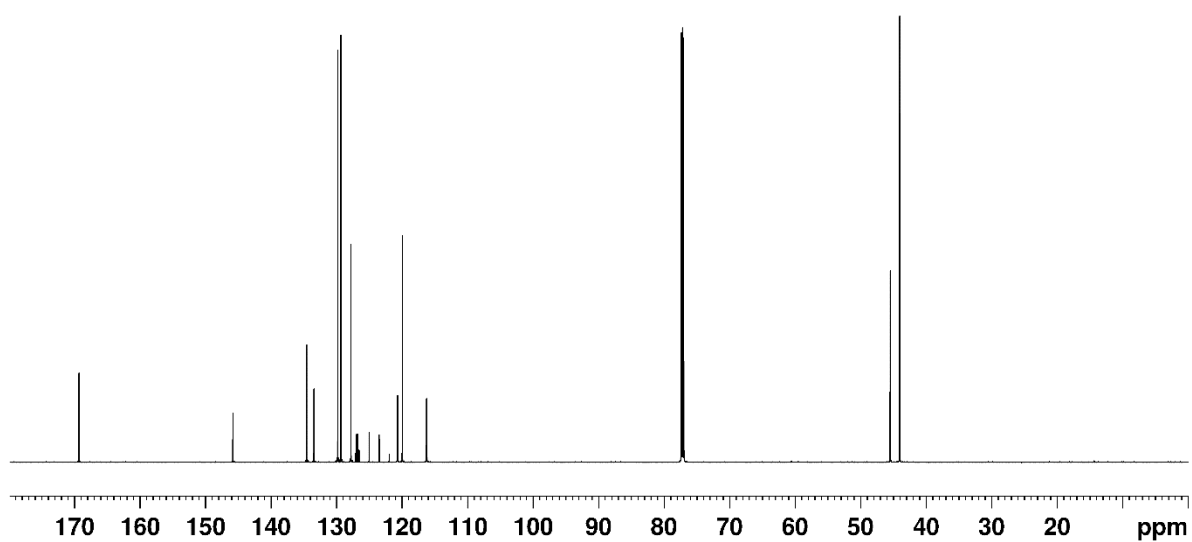
13 C NMR spectrum of 5 in CDCl 3
