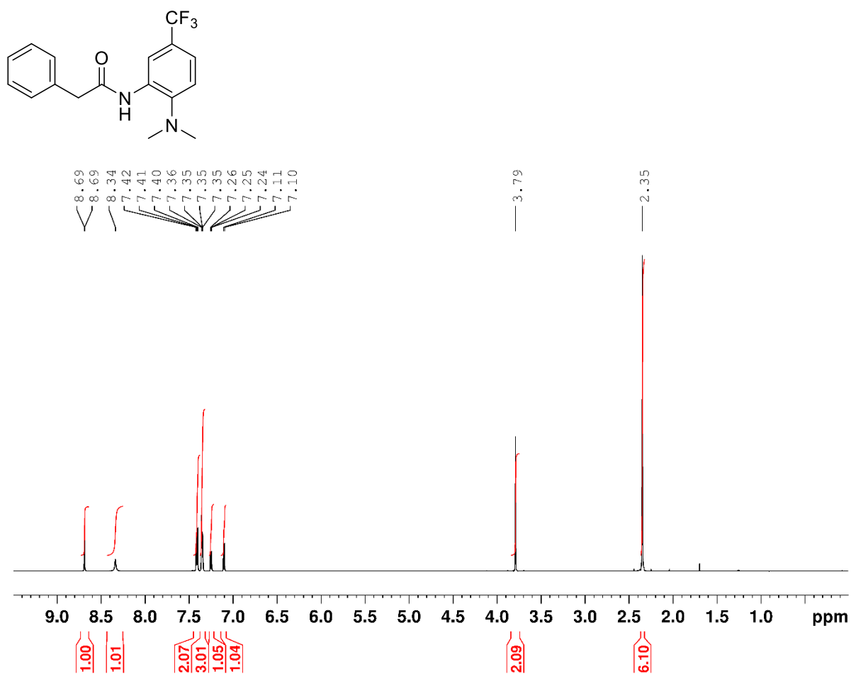
1 H NMR spectrum of 5 in CDCl 3
