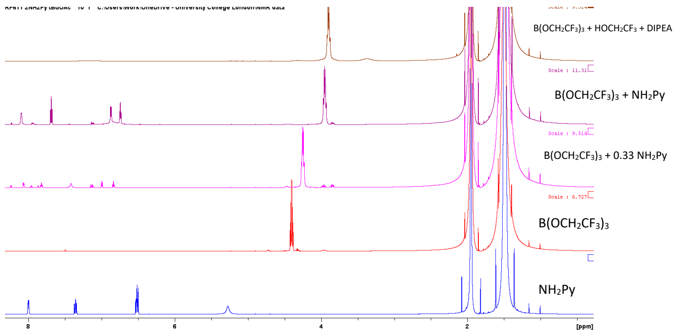
^1\text{H} NMR spectra of the indicated samples in t BuOAc
