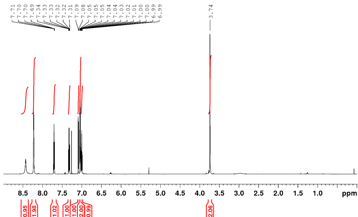
1 H NMR spectrum of 4 in CDCl 3
