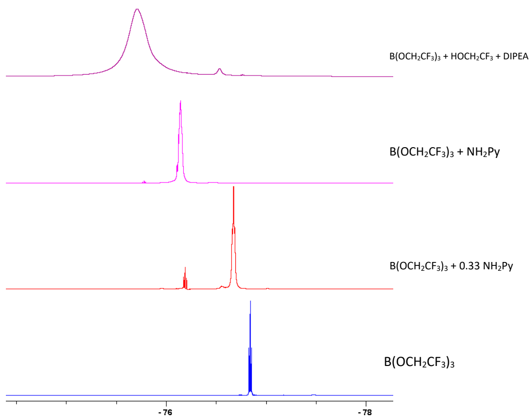
^{19}\text{F} NMR spectra of the indicated samples in t\text{BuOAc} .
