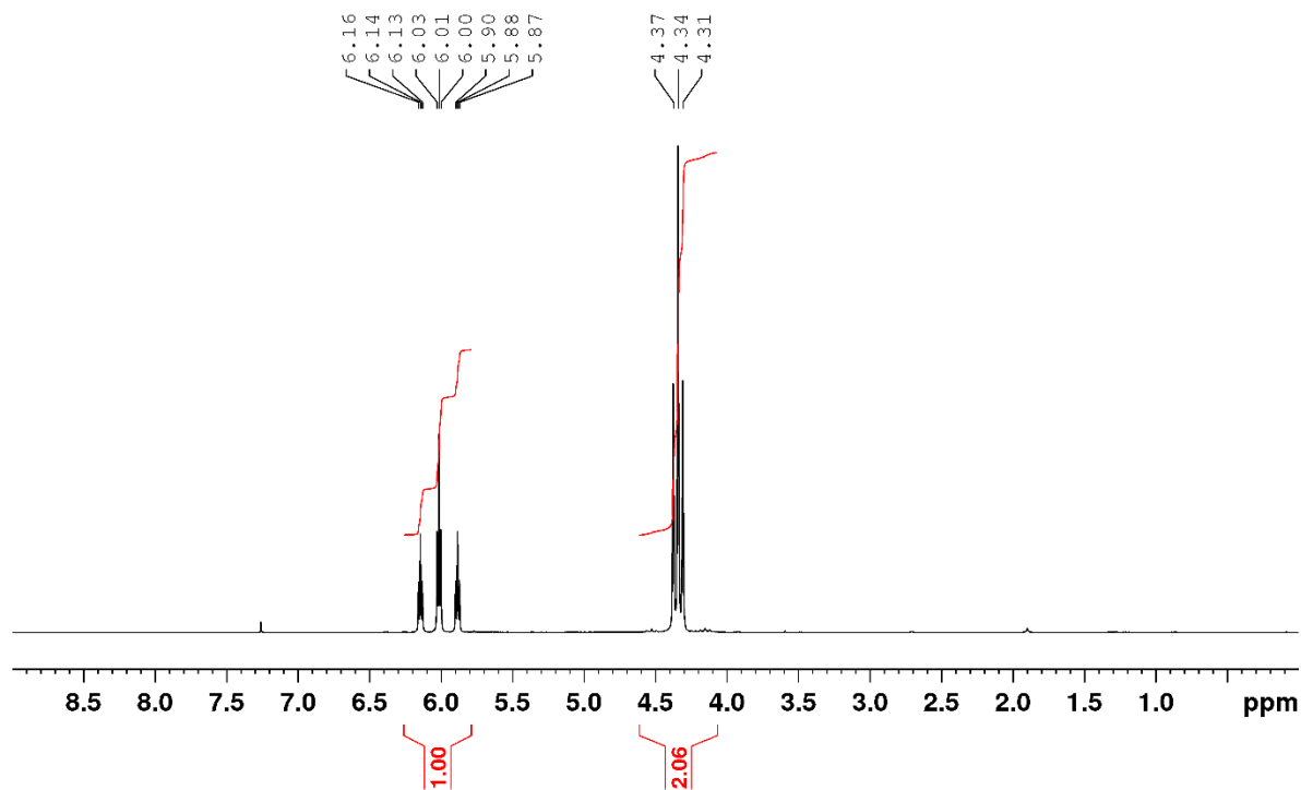
^1\text{H} NMR spectrum of \text{B}(\text{OCH}_2(\text{CF}_2)_3\text{CF}_2\text{H})_3 in \text{CDCl}_3 .
