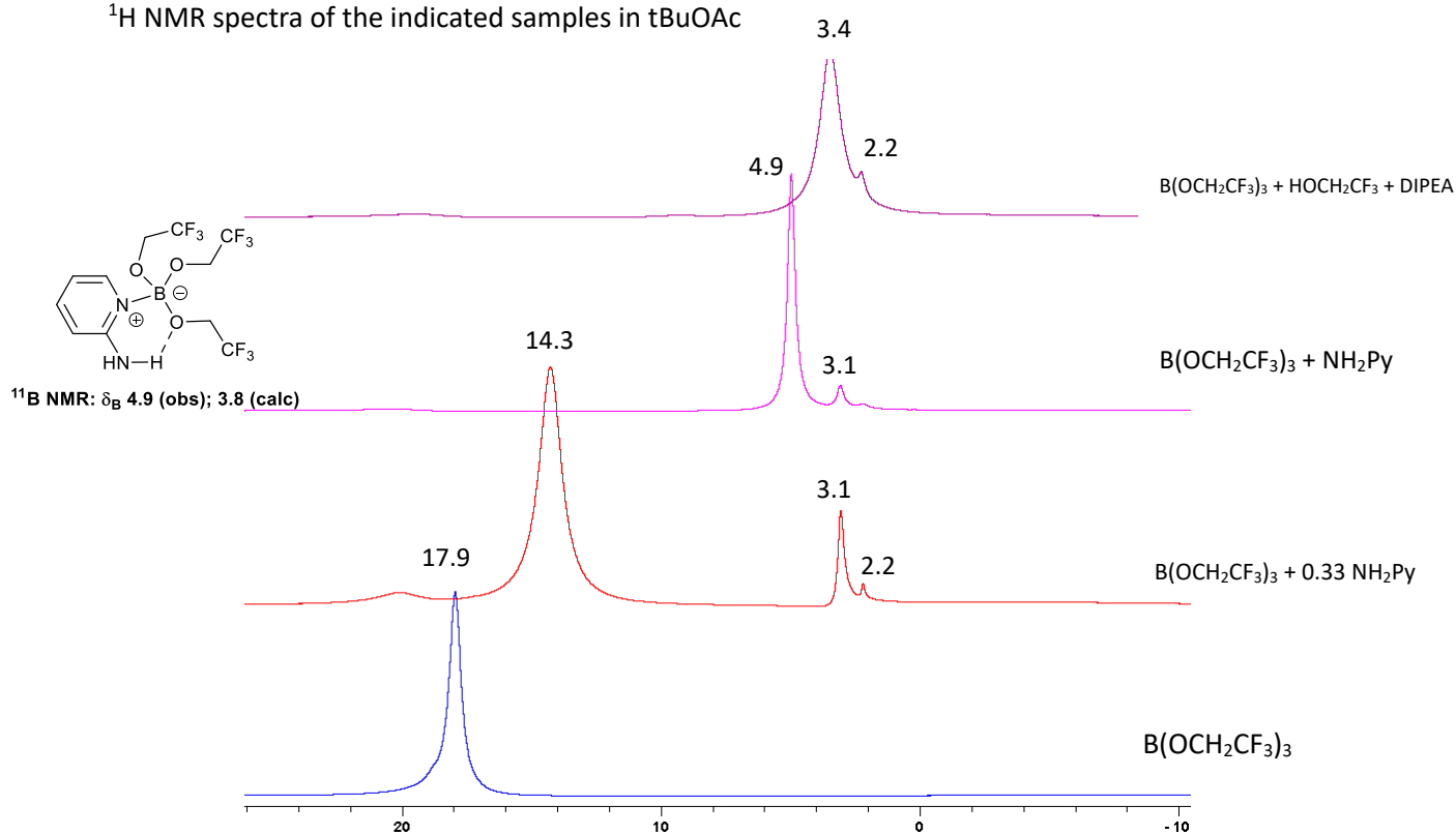
^{11}\text{B} NMR spectra of the indicated samples in t BuOAc.
