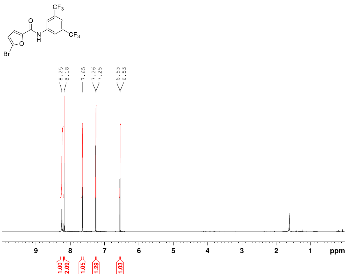
1 H NMR spectrum of 20 in CDCl 3
