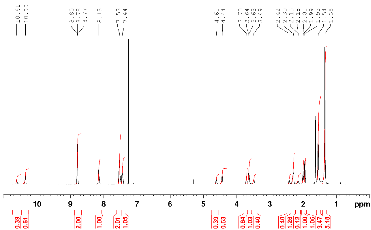
1 H NMR spectrum of 29 in CDCl 3
