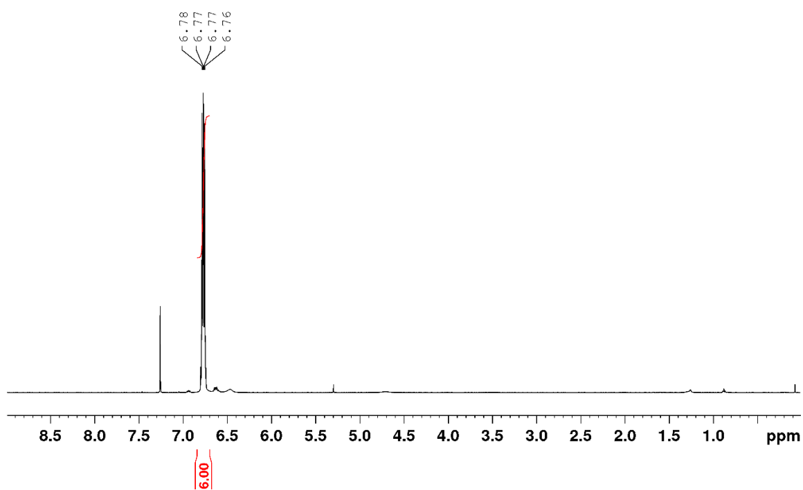
^1\text{H} NMR spectrum of \text{B}(\text{OAr}^{\text{F}})_3 in \text{CDCl}_3
