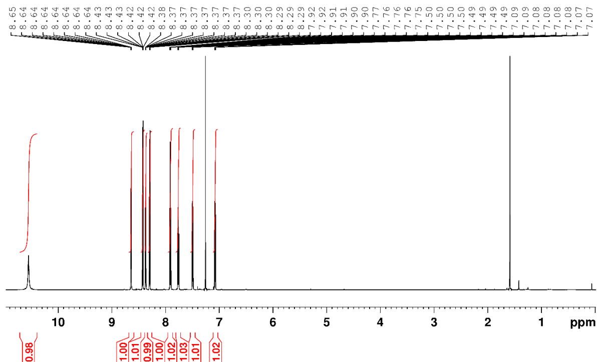
1 H NMR spectrum of 35 in CDCl 3
