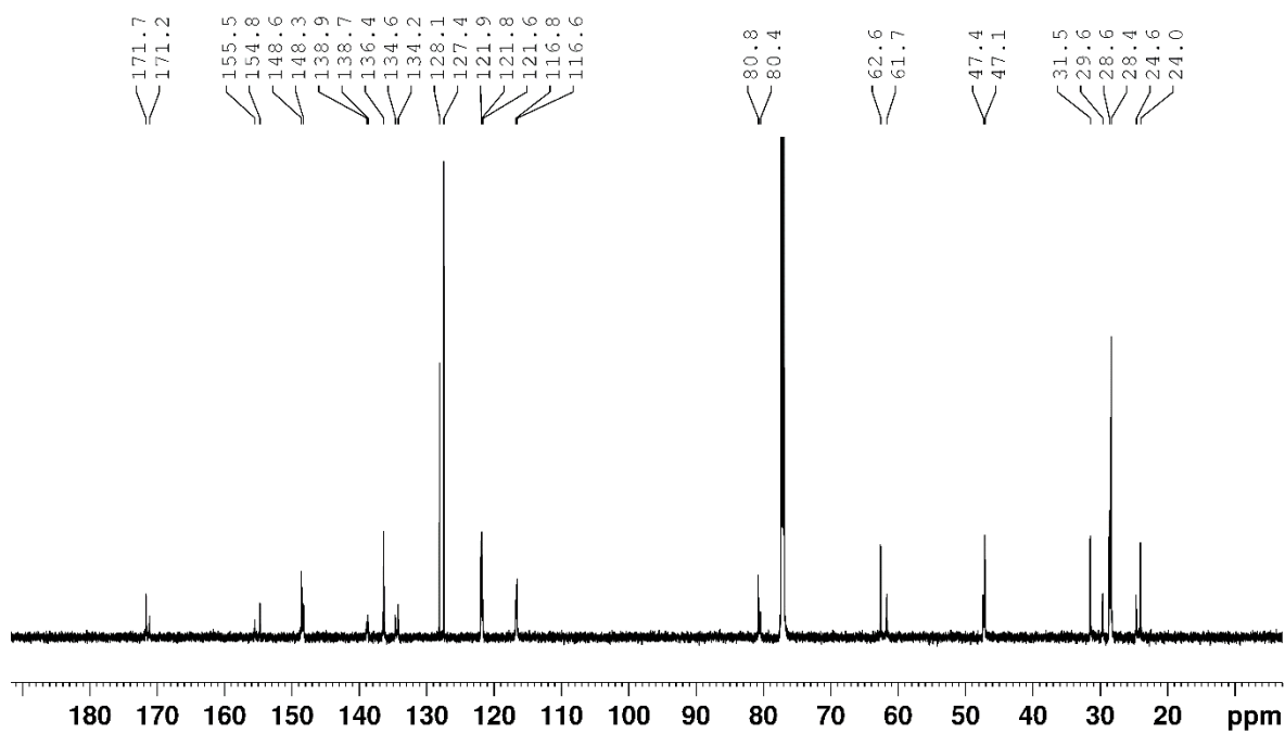
13 C NMR spectrum of 29 in CDCl 3
