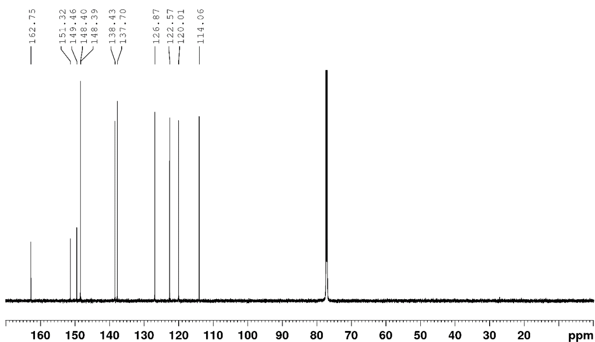
13 C NMR spectrum of 35 in CDCl 3 .
