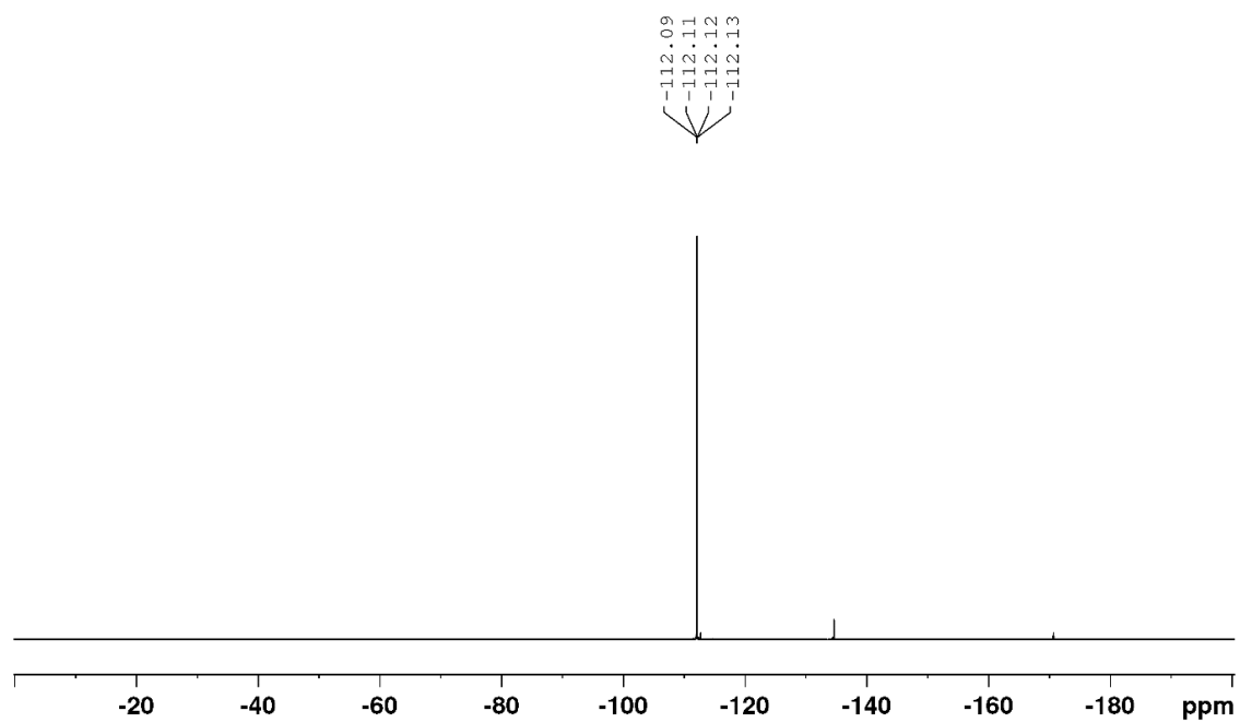
^{19}\text{F} NMR spectrum of 4 in \text{CDCl}_3
