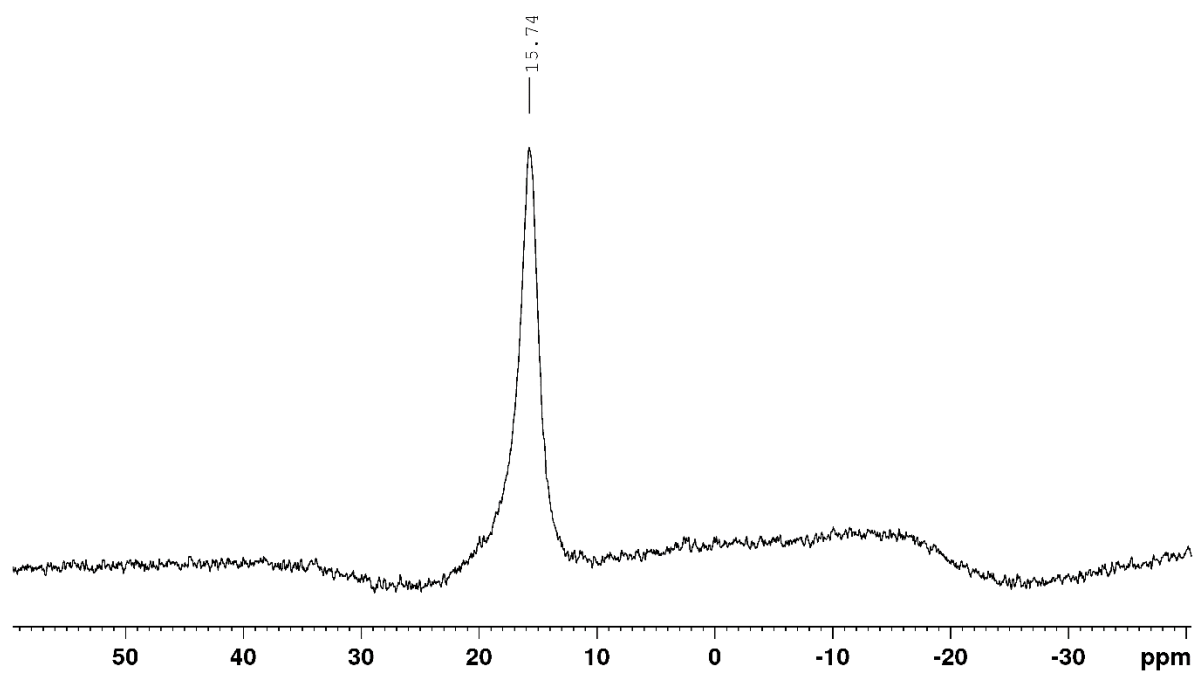
^{11}\text{B} NMR spectrum of \text{B}(\text{OAr}^{\text{F}})_3 in \text{CDCl}_3
