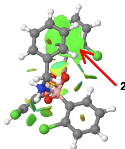
2-aminopyridine conformer
