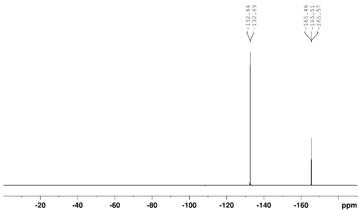
^{19}\text{F} NMR spectrum of \text{B}(\text{OAr}^{\text{F}})_3 in \text{CDCl}_3 .
