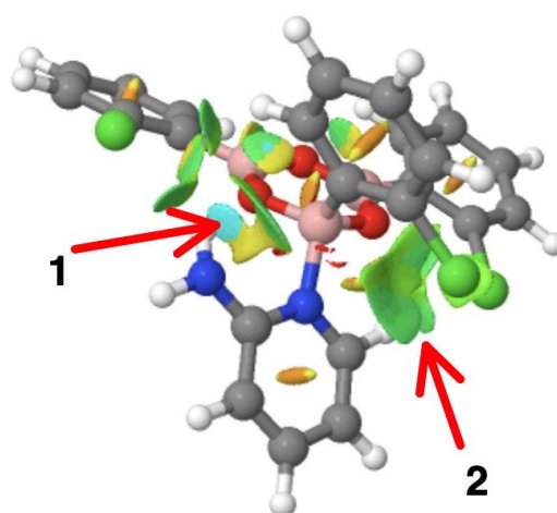
2-aminopyridine conformer
