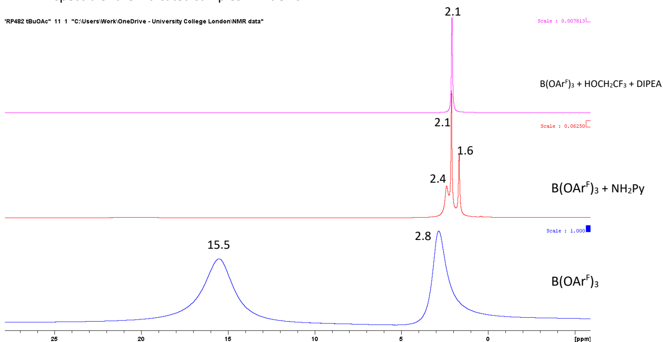
^{11}\text{B} NMR spectra of the indicated samples in t\text{BuOAc} .
