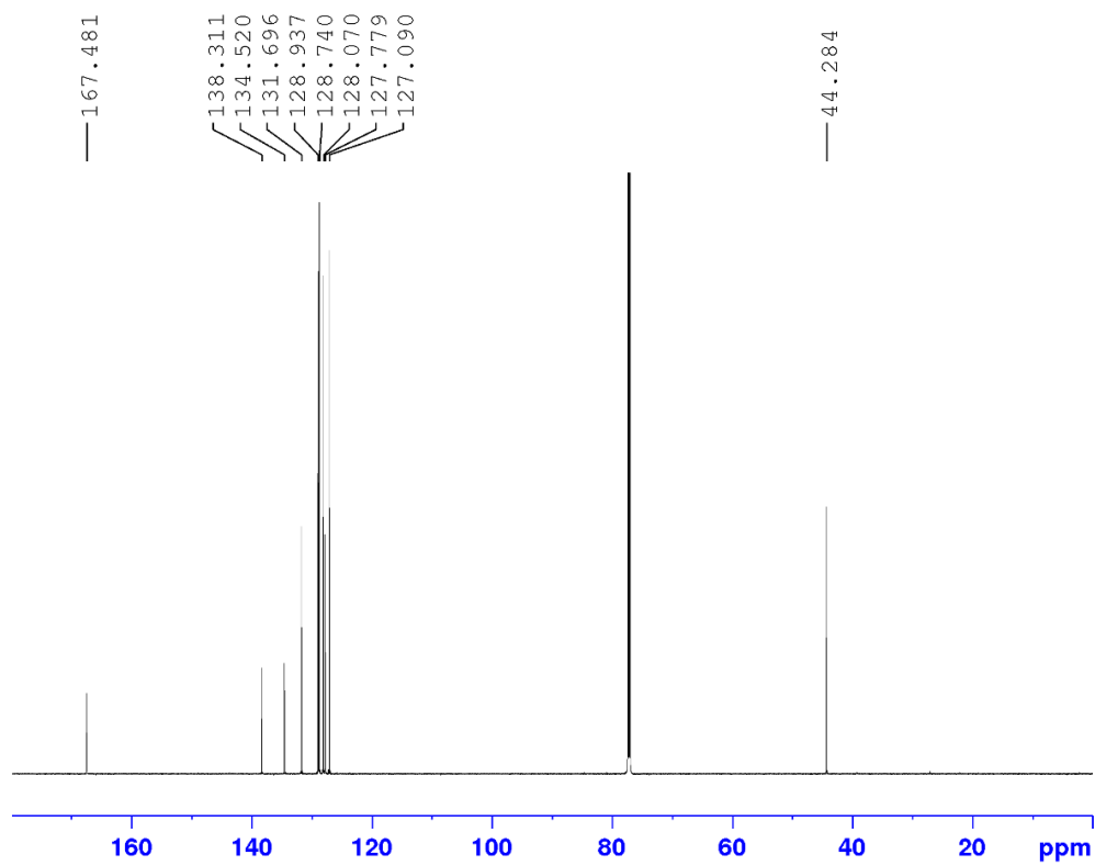
13 C NMR spectrum of 3 in CDCl 3
