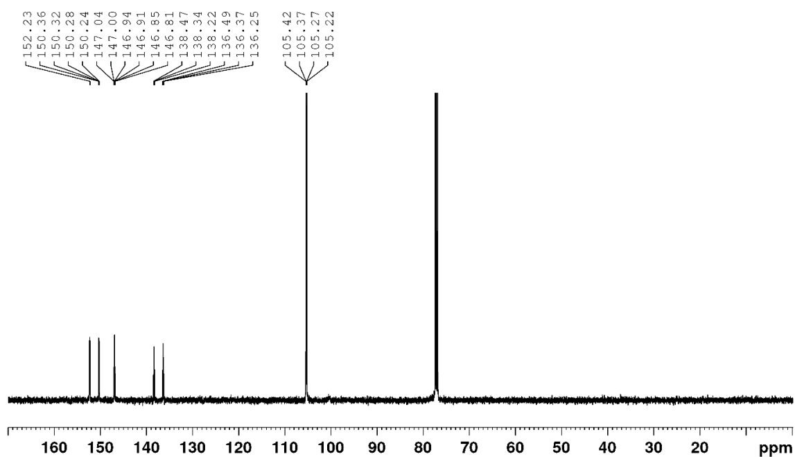
^{13}\text{C} NMR spectrum of \text{B}(\text{OAr}^{\text{F}})_3 in \text{CDCl}_3
