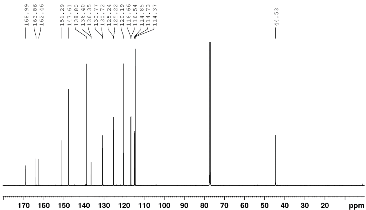
13 C NMR spectrum of 4 in CDCl 3
