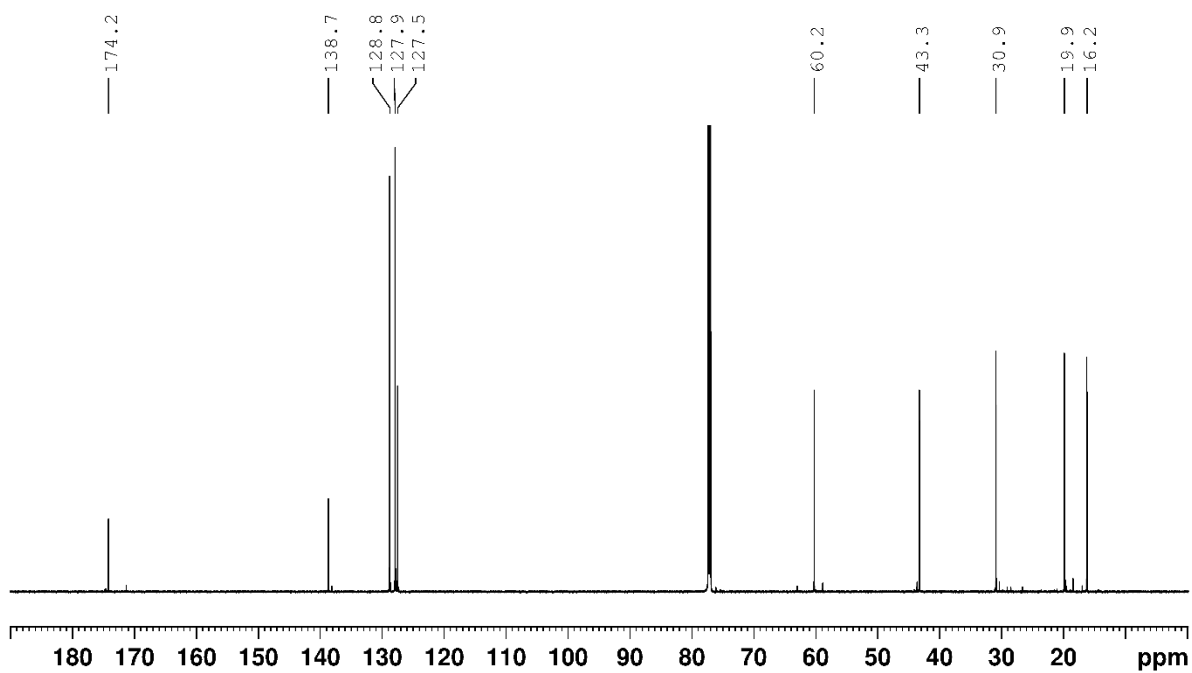
13 C NMR spectrum of 30 in CDCl 3
