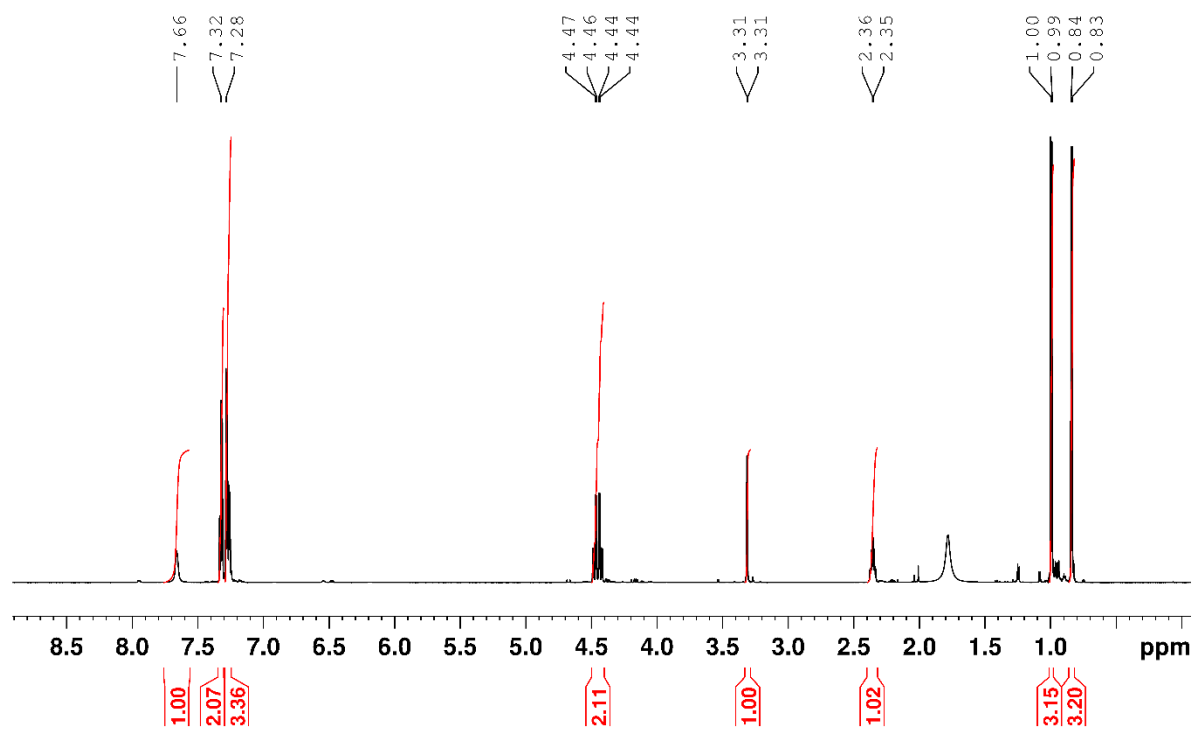
1 H NMR spectrum of 30 in CDCl 3
