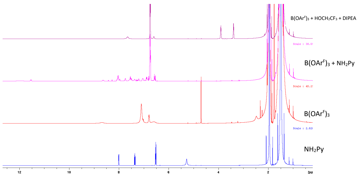
^1\text{H} NMR spectra of the indicated samples in t\text{BuOAc} .
