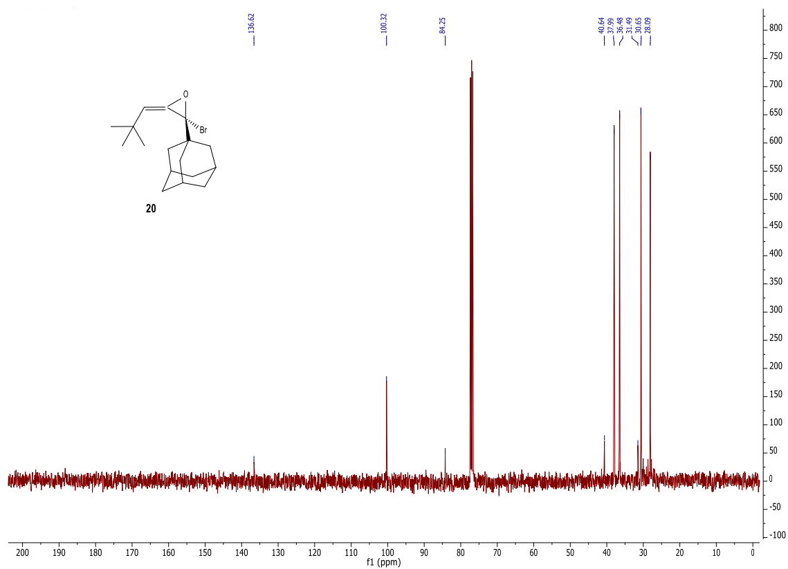
^{13}\text{C} NMR spectrum of E -1-adamantan-1-yl-1-bromo-1,2-epoxy-4,4-dimethyl-2-pentene ( 20 ) (100 MHz, \text{CDCl}_3 )
