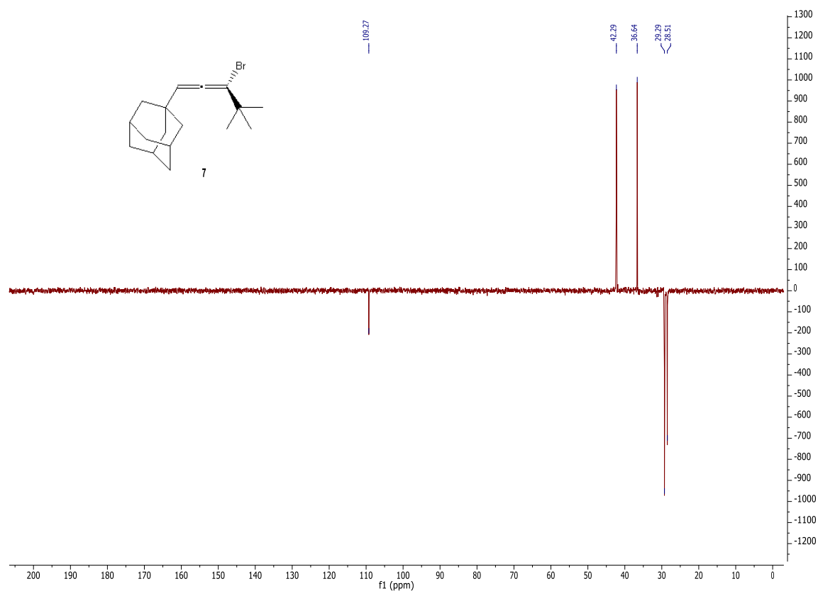
Selective (5.09 ppm) NOE spectrum of 1-adamantan-1-yl-3-bromo-4,4-dimethyl-1,2-pentadiene ( 7 ) (400 MHz, CDCl 3 )
