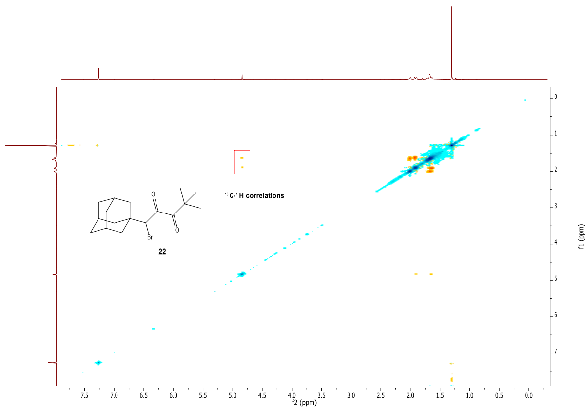
Bromine-induced isotopic shift in ^{13}\text{C} NMR spectrum of 1-adamantan-1-yl-1-bromo-4,4-dimethyl-2,3-pentanedione ( 22 ) (125 MHz, \text{CDCl}_3 ) 5
