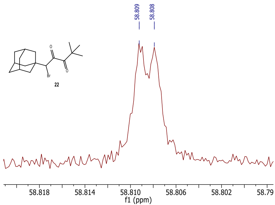
Bromine-induced isotopic shift in ^{13}\text{C} NMR spectrum of 1-adamantan-1-yl-1-bromo-4,4-dimethyl-2,3-pentanedione ( 22 ) (125 MHz, \text{CDCl}_3 ) 5
