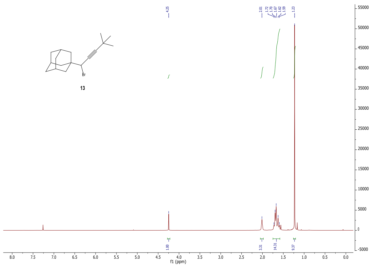
^1\text{H} NMR spectrum of 1-adamantan-1-yl-1-bromo-4,4-dimethyl-2-pentyne ( 13 ) (400 MHz, \text{CDCl}_3 )
