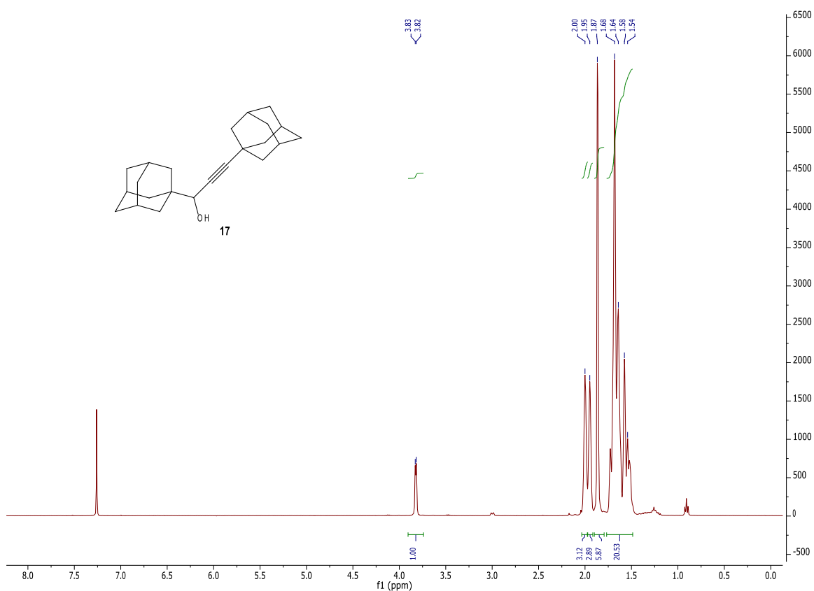
^1\text{H} NMR spectrum of 1,3-diadamantan-1-yl-2-propyn-1-ol ( 17 ) (400 MHz, \text{CDCl}_3 )
