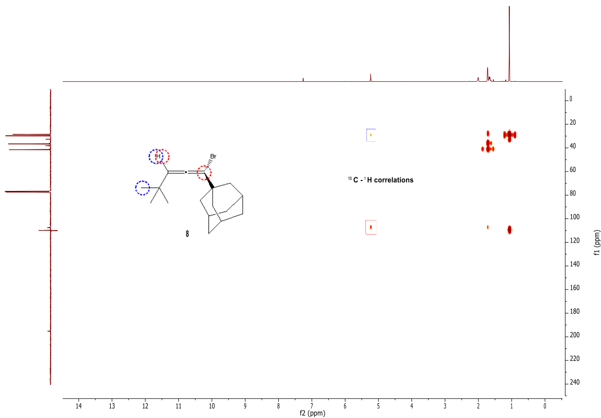
HMBC spectrum of 1-adamantan-1-yl-1-bromo-4,4-dimethyl-1,2-pentadiene ( 8 ) (400 MHz, CDCl 3 )
