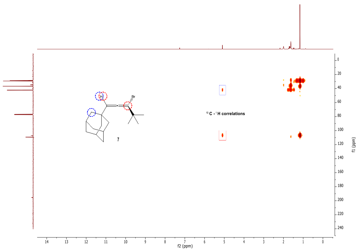
^1\text{H} NMR spectrum of 1-adamantan-1-yl-1-bromo-4,4-dimethyl-2-pentyne ( 13 ) (400 MHz, \text{CDCl}_3 )
