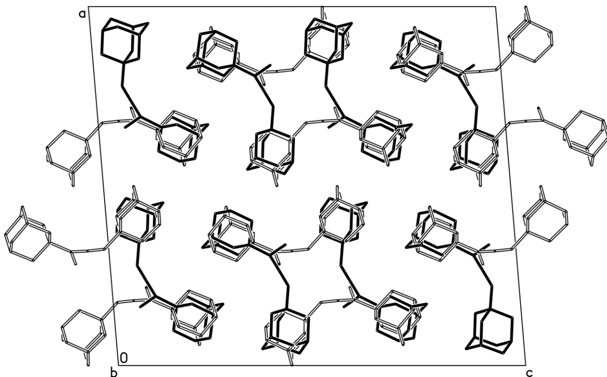
Fig. S2 Part of the extended packing in the crystal structure of 9 (viewed in parallel projection along the b axis direction), showing how the two disordered orientations exist in pairs that have very similar molecular shapes (the major and minor occupancy orientations have been drawn with dark and open bonds respectively).
