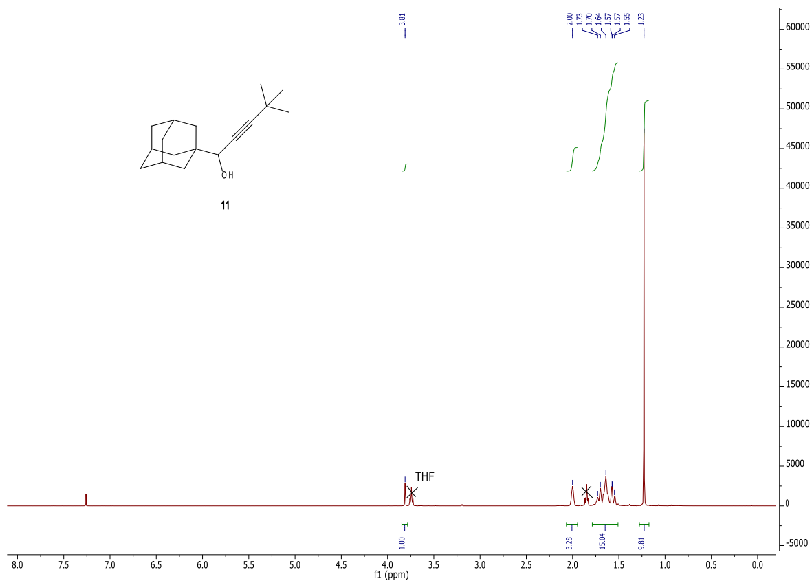
^{13}\text{C} NMR spectrum of 1-adamantan-1-yl-4,4-dimethyl-2-pentyn-1-ol ( 11 ) (100 MHz, \text{CDCl}_3 )
